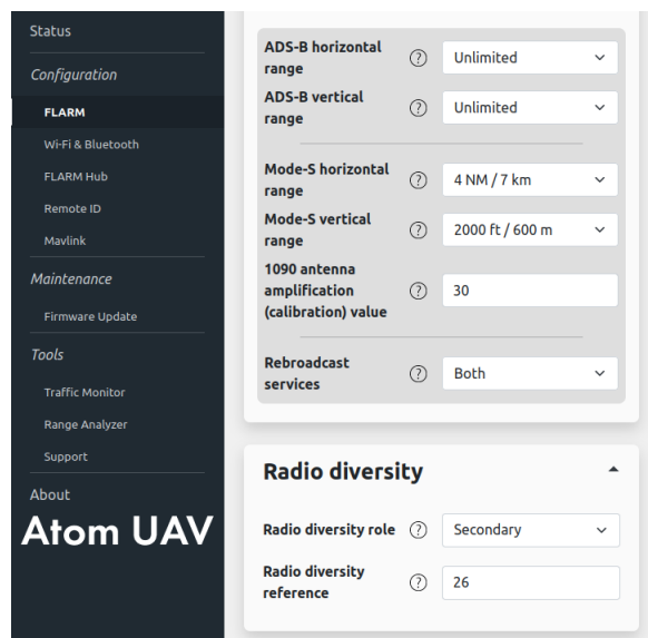
Setting radio diversity role in secondary device
